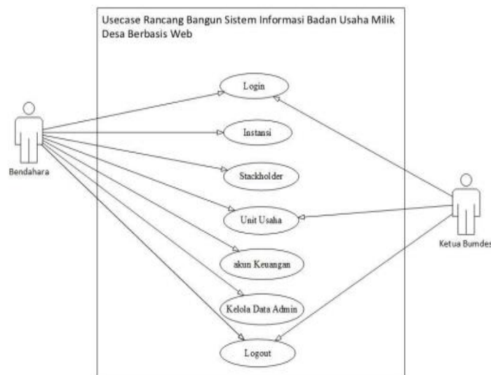
Gambar 2. Usecase Diagram
